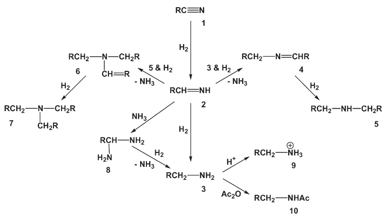
SCHEME 1 Reaction mechanism of nitrile hydrogenation to primary amines
