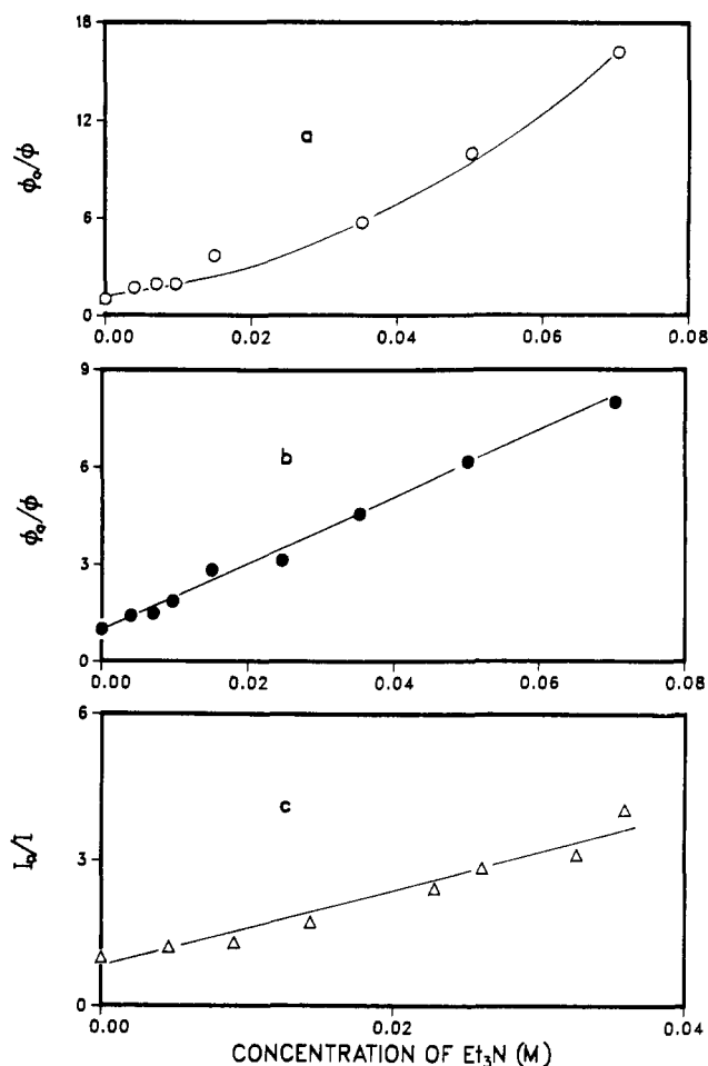
Figure 4. Stern-Volmer plots of the quenching of the quantum yields of furanyl ether 7 (a) and furanyl ether 6 (b) and of fluorescence intensities of 2 (c), by Et_3N in benzene.
