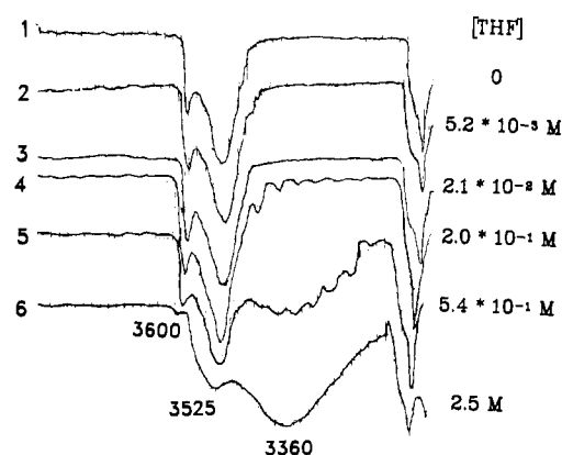
Figure 6. IR absorptions (3000–4000- \text{cm}^{-1} range) of allylnaphthol 1 in \text{CCl}_4 in the presence of increasing amounts of tetrahydrofuran: [THF] 0 ( 1 ), 5.2 \times 10^{-3} ( 2 ), 2.1 \times 10^{-2} ( 3 ), 2 \times 10^{-1} ( 4 ), 5.4 \times 10^{-1} ( 5 ), and 2.5 M ( 6 ).
