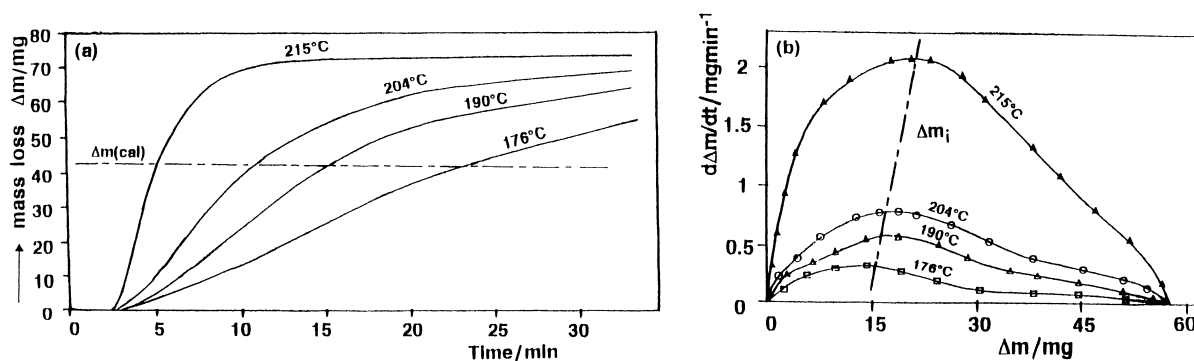
Fig. 3. \text{Cu}_3\text{Si} -Ref/ \text{CuCl} : (a) mass loss \Delta m vs. time and (b) rate \Delta m/dt vs. \Delta m .
