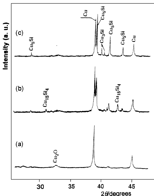
Fig. 6. X-ray diffraction patterns obtained after the reaction between \text{CuCl} and: (a) \text{Cu}_3\text{Si} -MASHS at 180°C; (b) \text{Cu}_3\text{Si} -M2AP at 190°C; (c) \text{Cu}_3\text{Si} -Ref at 230°C.
