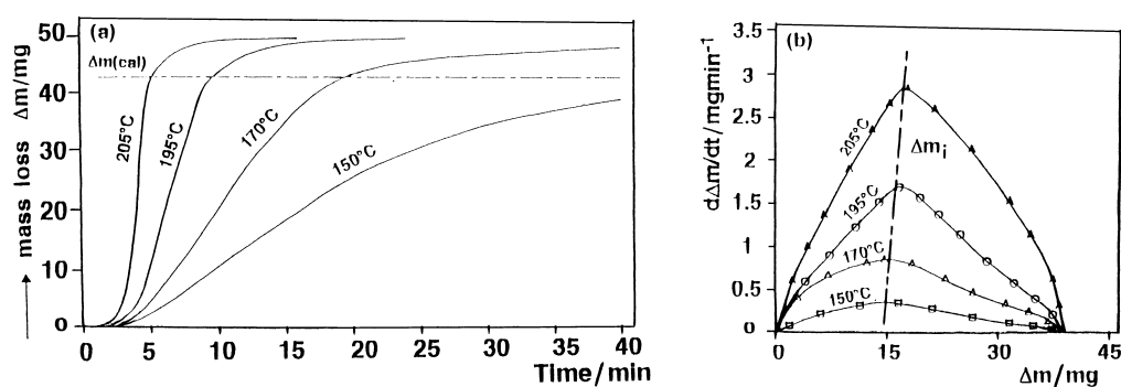
Fig. 4. \text{Cu}_3\text{Si} -M2AP/ \text{CuCl} : (a) mass loss \Delta m vs. time and (b) rate \Delta m/dt vs. \Delta m .
