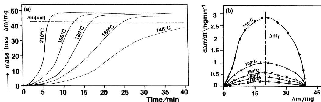
Fig. 5. \text{Cu}_3\text{Si} -MASHS/ \text{CuCl} : (a) mass loss \Delta m vs. time and (b) rate \Delta m/\text{dt} vs. \Delta m .
