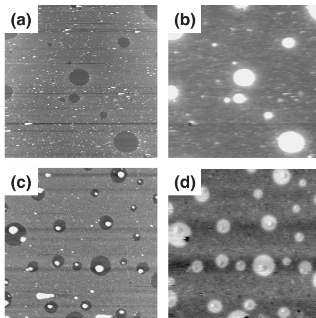
Figure 1. AFM ((a) and (c)) and KFM ((b) and (d)) images ( 20 \times 20 \mu\text{m}^2 ) of functionalized templates before ((a) and (b)) and after ((c) and (d)) immersion in aqueous \text{Zr}(\text{SO}_4)_2 solution at room temperature for 6 h.
