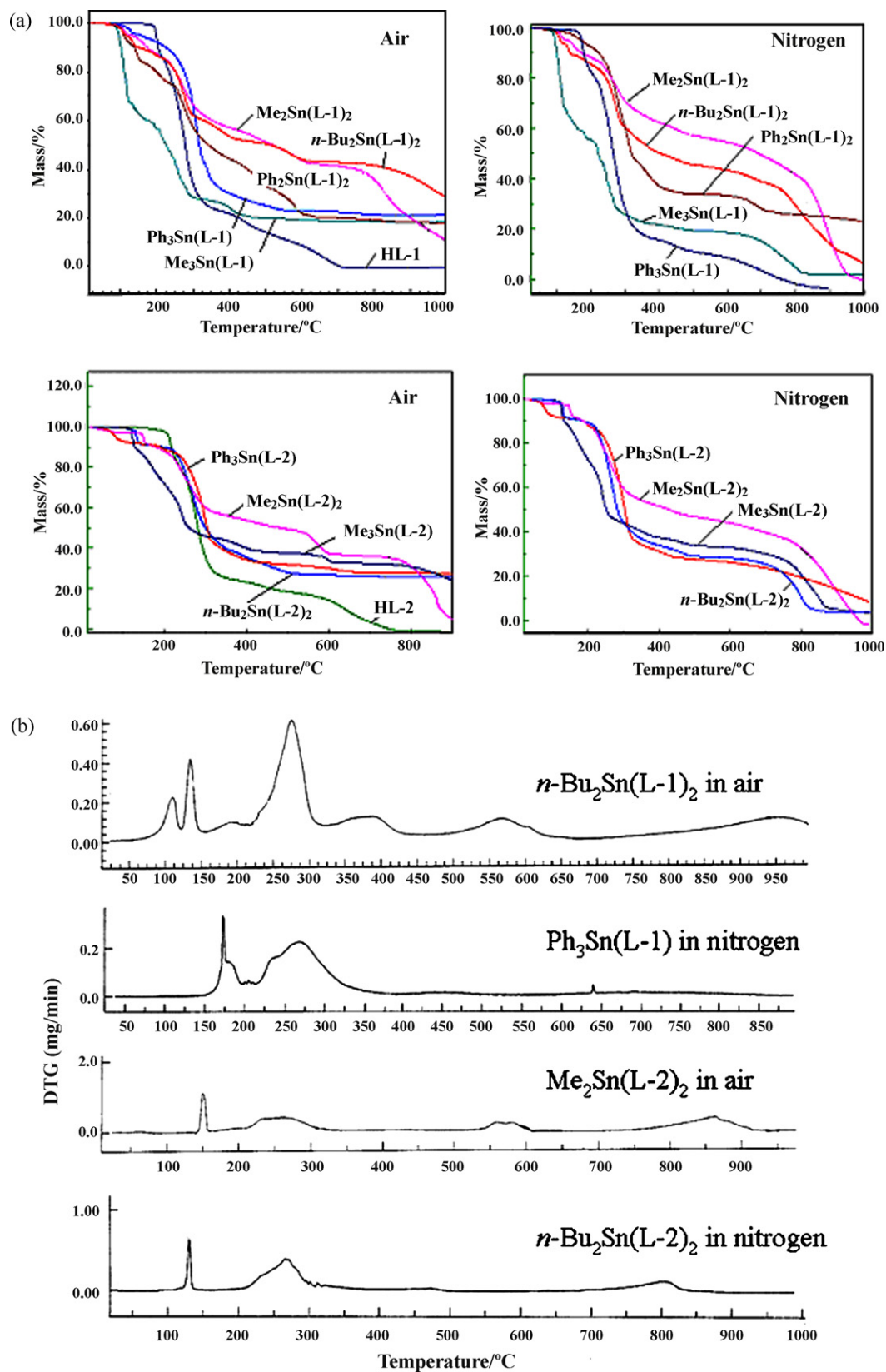
Fig. 2. (a) TGA plots of HL-1, HL-2 in air, and their diorganotin(IV) triazolates and triorganotin(IV) triazolates under air and nitrogen. (b) DTG plots of n -Bu 2 Sn(L-1) 2 and Me 2 Sn(L-2) 2 under air and n -Bu 2 Sn(L-2) 2 and Ph 3 Sn(L-1) under nitrogen.
