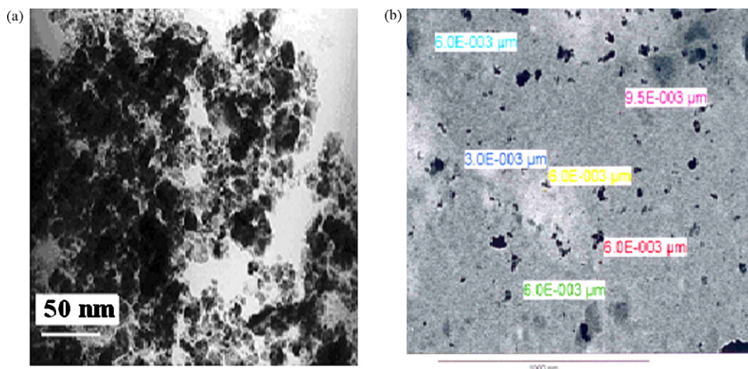
Fig. 7. TEM image of residues obtained by thermal decomposition of n\text{-Bu}_2\text{Sn}(\text{L-1})_2 in nitrogen (a); n\text{-Bu}_2\text{Sn}(\text{L-2})_2 in air (b).
