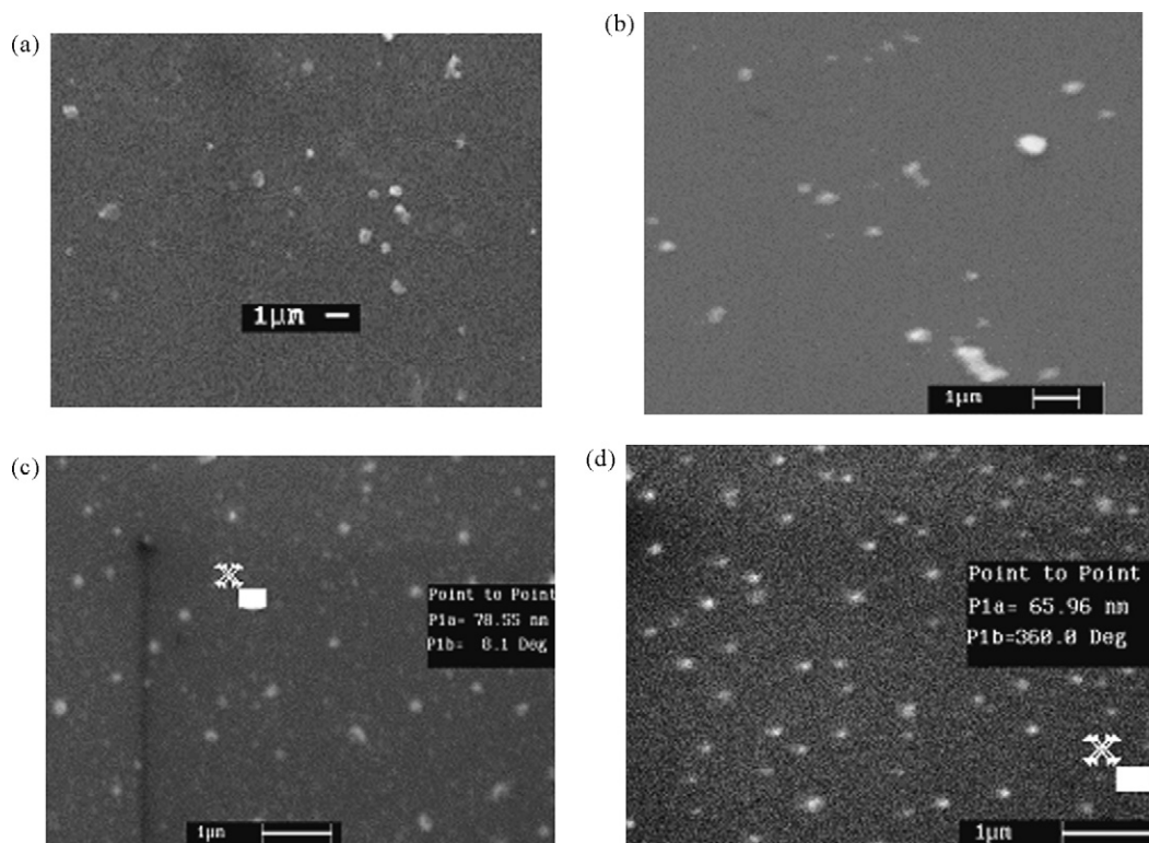
Fig. 6. SEM image of residues obtained by thermal decomposition of \text{Ph}_3\text{Sn}(\text{L-1}) in air (a); n\text{-Bu}_2\text{Sn}(\text{L-1})_2 in nitrogen (b); n\text{-Bu}_2\text{Sn}(\text{L-2})_2 in air (c); and \text{Ph}_3\text{Sn}(\text{L-2}) in nitrogen (d).
