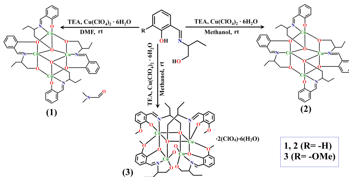
Scheme 1. Synthesis of complexes 1-3 .
