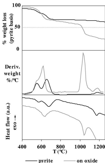
Fig. 1. Weight loss (in pyrite basis), DGTa curves and heat flow profiles of thermal decomposition of pyrite and pyrite laid on an hematite disc.
