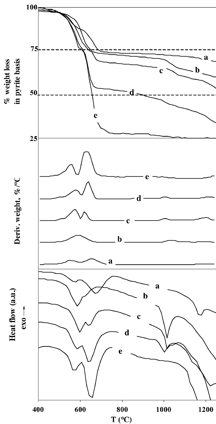
Fig. 3. Weight loss in pyrite weight basis, DGT curves and heat flow profiles of thermal evolution of pyrite and its mixtures with hematite. a: pure pyrite; b: 50% pyrite; c: 33% pyrite; d: 17% pyrite; e: 8% pyrite.
