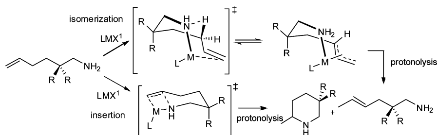
Scheme 3. Reaction Products from the Hydroamination/Cyclization of 1-Amino-5-hexenes with 1a
