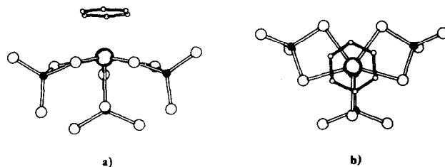
Figure 2. Projections of the molecule in the plane of the benzene ring, b), and in a plane nearly perpendicular, a).
