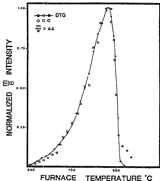
Fig. 3. Decomposition of \text{CaCO}_3 studied by the TA-MS combination. Sample, 100 mg \text{CaCO}_3 (Hopkin and Williams); sample holder, cylindrical alumina crucible; furnace atmosphere, flowing argon ( 50 \text{ ml min}^{-1} ); heating rate, 6^\circ\text{C min}^{-1} .
