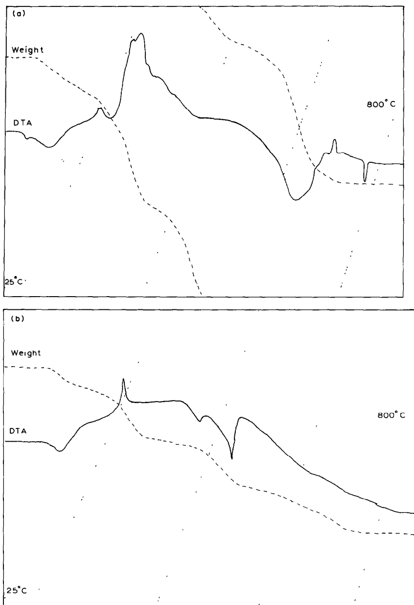
Fig. 1. TG (---) and DTA (—) curves for (a) \text{Fe(OH)}_3(\text{nic}) \cdot 0.75\text{H}_2\text{O} and (b) \text{Fe(OH)}_2(\text{isonic}) \cdot \text{H}_2\text{O} . Linear heating is also shown.
