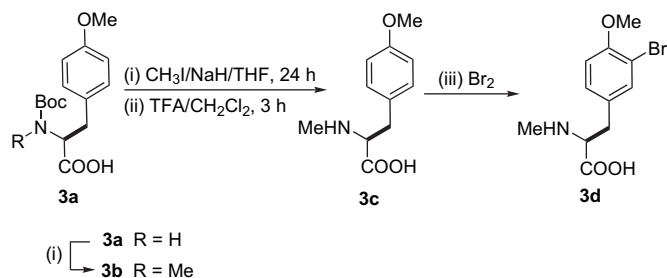
Scheme 1. Synthesis of standard N,O -diMe-3'-Br- L -Tyr ( 3d ).
