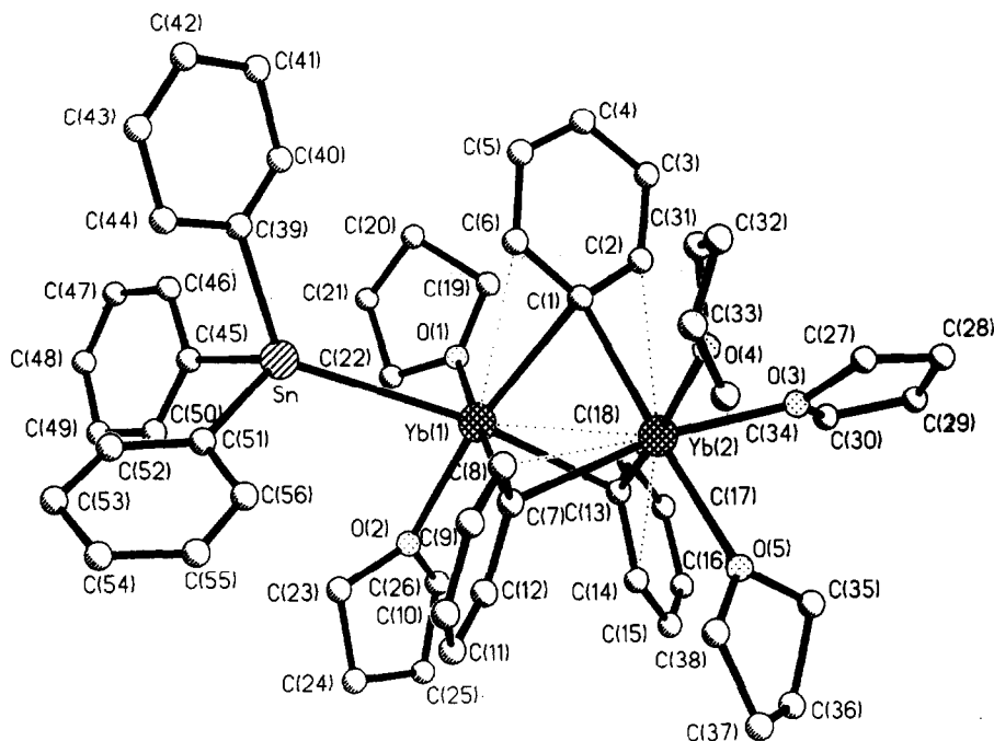
Fig. 1. Molecular structure of \text{Ph}_3\text{SnYb(THF)}_2(\mu\text{-Ph})_3\text{Yb(THF)}_3 with atom labels.
