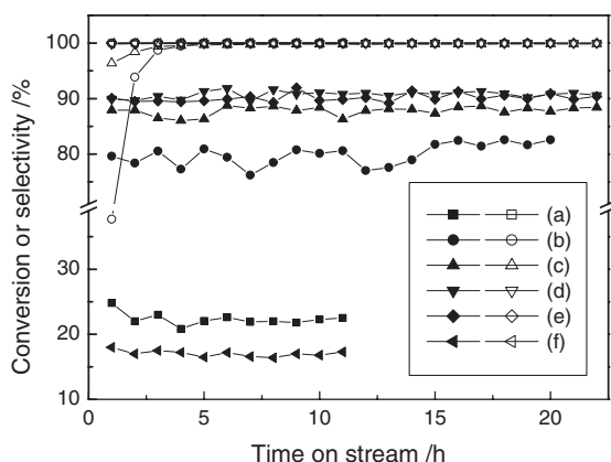
Figure 1. Methanol dehydration to DME over various solid acid catalysts ( T = 250^\circ\text{C} , P = 10 atm, LHSV = 4.8\text{ h}^{-1} , symbol: solid = conversion of MeOH and open = selectivity to DME, \gamma - \text{Al}_2\text{O}_3 (a) and double layer bed [ \gamma - \text{Al}_2\text{O}_3 (top, 2.6 g) + \text{Na}_x -H-ZSM-5 (bottom, 0.54 g)] with mol % Na = 10 (b), = 20 (c), = 40 (d), = 80 (e) and = 100 (f).
