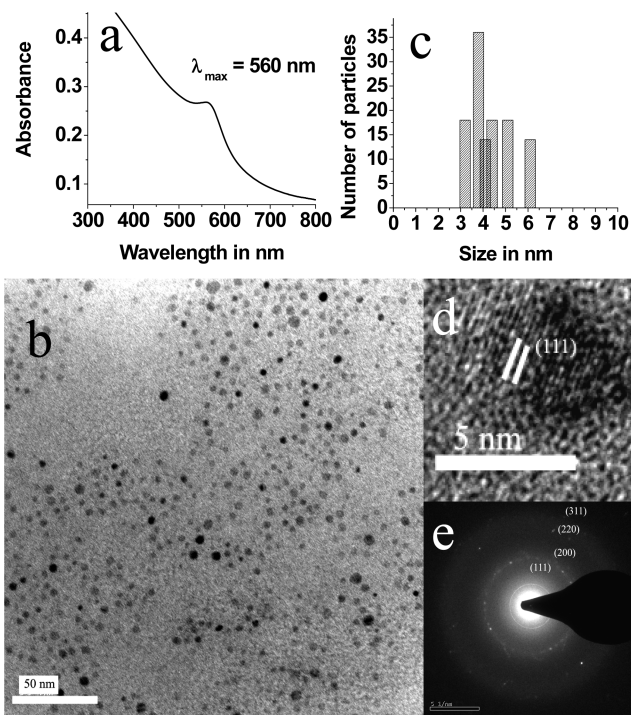
Figure 9. (a) UV–visible spectrum of Cu colloid. (b) TEM bright field image of Cu colloid. (c) Histogram showing the particle size distribution. (d) HRTEM image of Cu(0) nanoparticle. (e) SAED pattern of Cu(0) nanoparticles.
