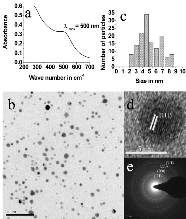
Figure 11. (a) UV–visible spectrum of Au colloid. (b) TEM bright field image of Au colloid. (c) Histogram showing the particle size distribution. (d) HRTEM image of Au(0) nanoparticle. (e) SAED pattern of Au(0) nanoparticles.
