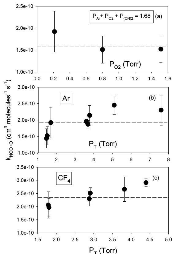
Figure 5. k_1 independence (a) from \text{O}_2 and likely \text{NO}(\text{v}) , see text. The total pressure was constant at 1.68 Torr, and the \text{P}_{\text{O}_2} varied. Each data point is the average of 3–5 measurements of k_1 obtained by varying the ArF fluence, and the error bars are \pm 1\sigma from the average. The dashed line is the average of the data weighted by the number of measurements. Panel b provides the summary of the data for the determination of k_1 with Ar as carrier gas. Each data point is the average of 3–5 measurements of k_1 , as in panel a. The dashed line is the average of the data weighted by the number of measurements, giving k_1 = (1.94 \pm 0.30) \times 10^{-10} \text{ cm}^3 \text{ molecule}^{-1} \text{ s}^{-1} . The data indicate that k_1 is independent of Ar pressure. Panel c provides the summary of the data for the determination of k_1 with \text{CF}_4 as the carrier gas. As in panel b, the average of the data weighted by the number of measurements of k_1 gives k_1 = (2.37 \pm 0.34) \times 10^{-10} \text{ cm}^3 \text{ molecule}^{-1} \text{ s}^{-1} . The data indicate that k_1 is independent of \text{CF}_4 pressure.
