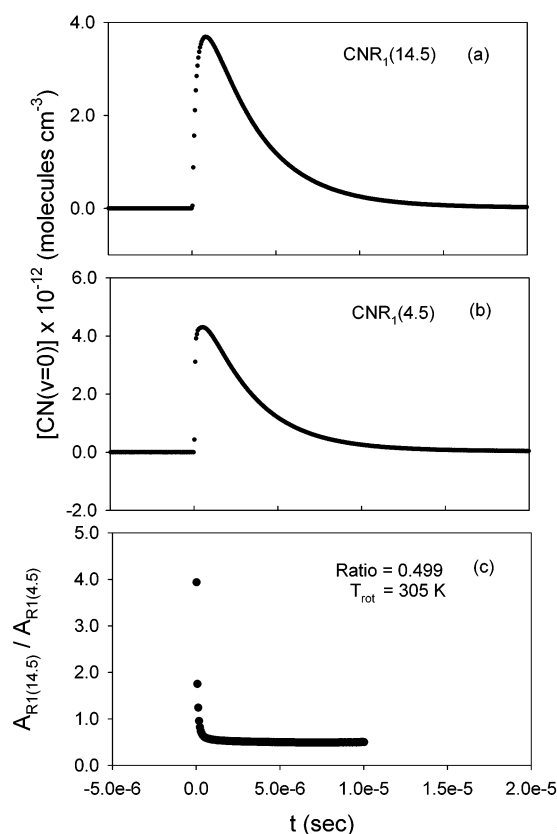
Figure 6. The temporal dependence of CN concentration determined (a) from monitoring the \text{R}_1(14.5) transition and (b) from monitoring the \text{R}_1(4.5) transition. The conditions of the experiment were \text{P}_{\text{Ar}} = 3.15 , \text{P}_{\text{O}_2} = 0.423 , and \text{P}_{(\text{CN})_2} = 0.190 Torr. Panel c shows the ratio of the absorbance profiles used to calculate the CN concentration profiles in panels a and b. The first point corresponds to a rotational temperature of \sim 1000 \text{ K} , and the plateau region corresponds to a rotational temperature of 305 \text{ K} . The temperature of the reaction vessel was 292 \text{ K} .
