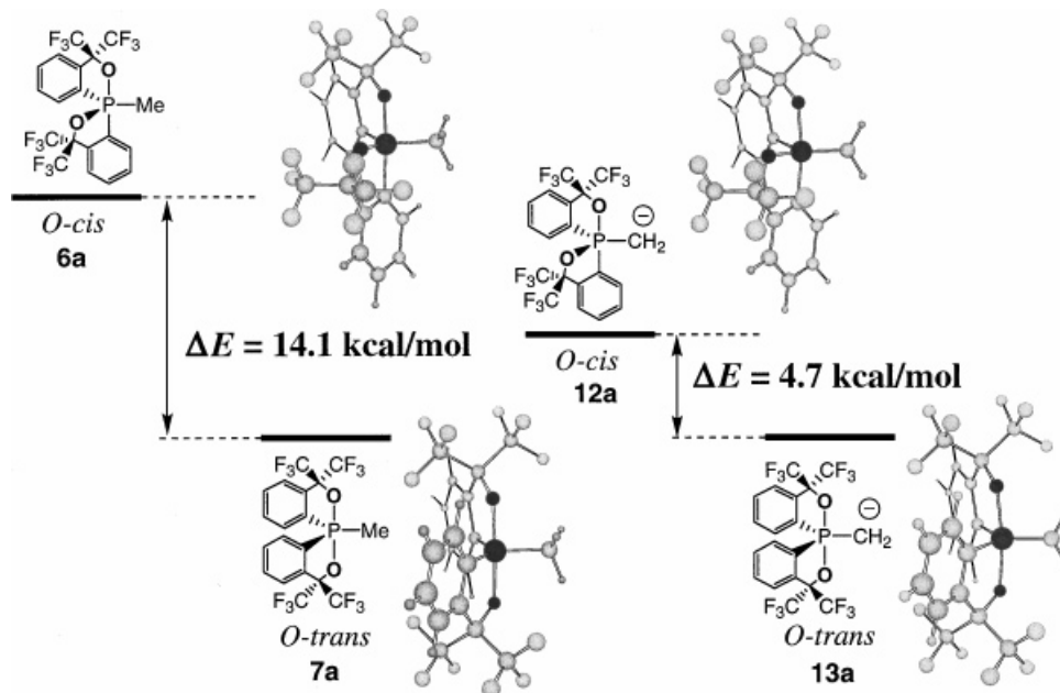
FIGURE 3 Decrease in energy difference between the anionic pair of O-cis 12a and O-trans 13a compared with the corresponding neutral pair of O-cis 6a and O-trans 7a attributable to n_{\text{C}} \rightarrow \sigma^*_{\text{P-O}} stabilization.
