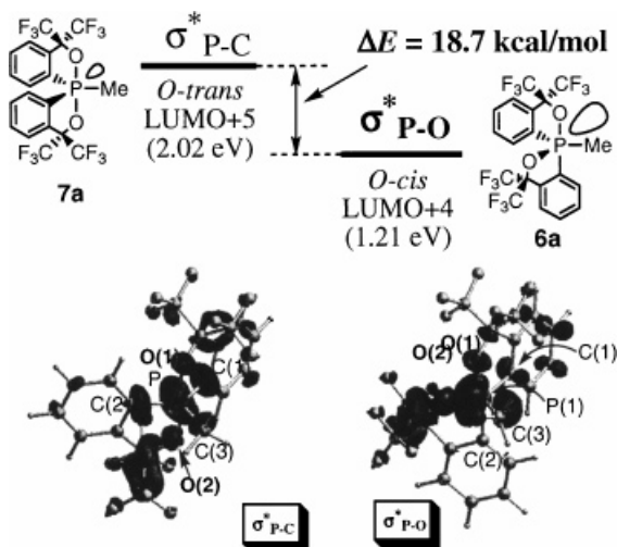
FIGURE 2 Energies of molecular orbitals for \sigma^*_{\text{P-O}} of O-cis 6a and \sigma^*_{\text{P-O}} of O-trans 7a .
