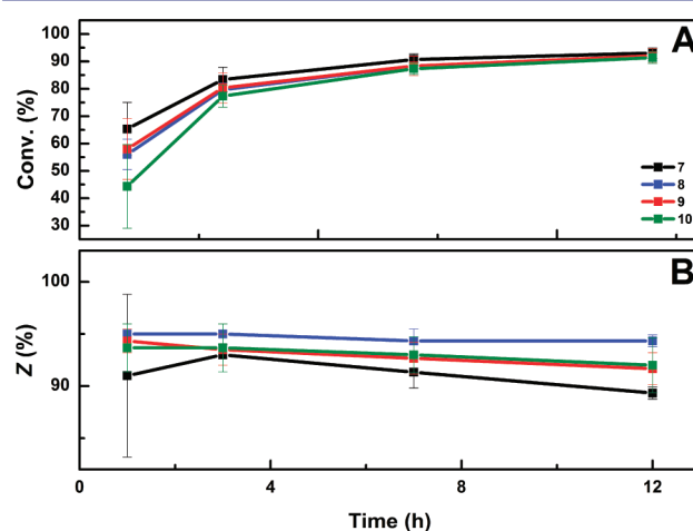
Figure 3. Time-course plot for the conversion (A) and selectivity (B) of homodimerization of 15 to 16 using catalysts 7–10 . Conditions were 15 (1 mmol) and catalyst (1 \mu mol) in THF (0.1 mL) at 35 ^{\circ} C. Data points and error bars were calculated from the average and standard deviation of three separate runs.
