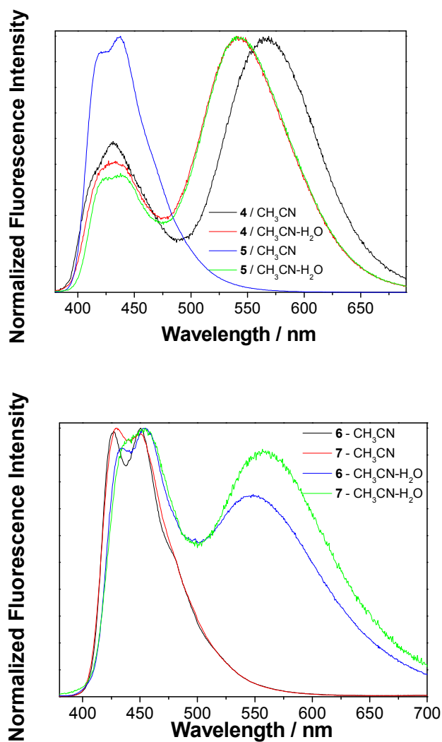
Fig 1. Normalized fluorescence spectra ( \lambda_{\text{exc}} = 370 \text{ nm} ) of 4 and 5 (top), and 6 and 7 (bottom) in \text{CH}_3\text{CN} or \text{CH}_3\text{CN-H}_2\text{O} (1:1).
