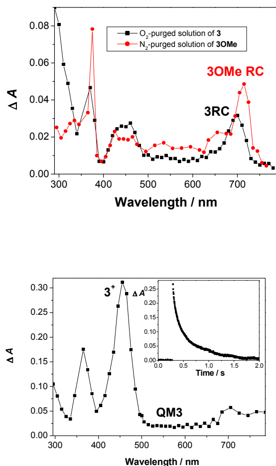
Fig 3. Transient absorption spectra of 3 and 3OMe in O_2 -purged CH_3CN or N_2 -purged CH_3CN - H_2O (1:1) collected 700 ns after the laser pulse (top) and in 1,1,1,3,3,3-hexafluoroisopropanol (HFIP) collected 760 ns after the laser pulse (bottom, weak \Delta A at 500-600 nm corresponds to QM3 , whereas the maximum at 450 nm corresponds to 3^+ ; inset: decay of 3^+ at 450 nm).
