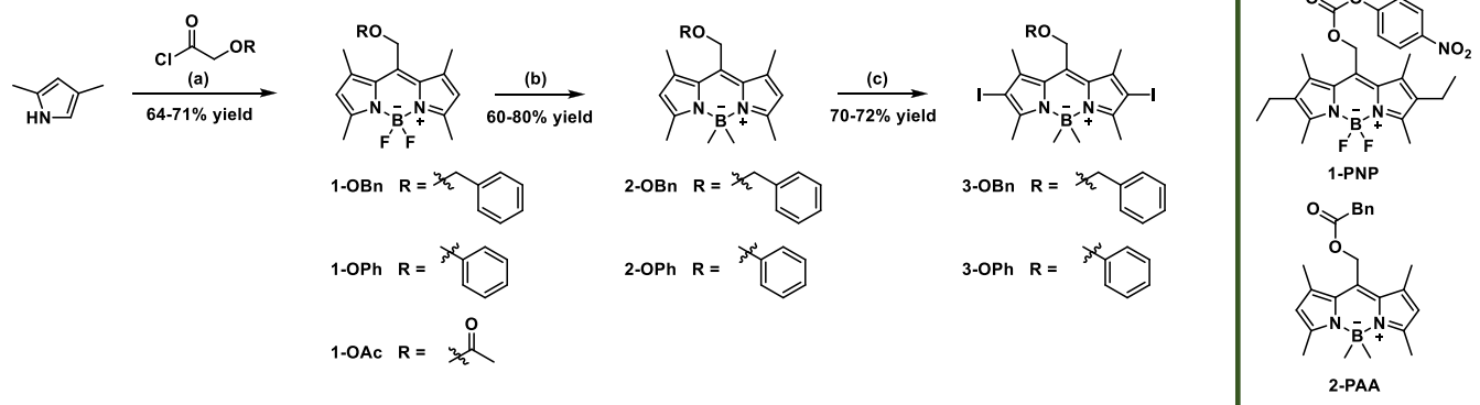
Scheme 1. Synthesis of BODIPY Compounds Ether Linkages from Acetyl Chlorides to Investigate the Release of Alcohols a
