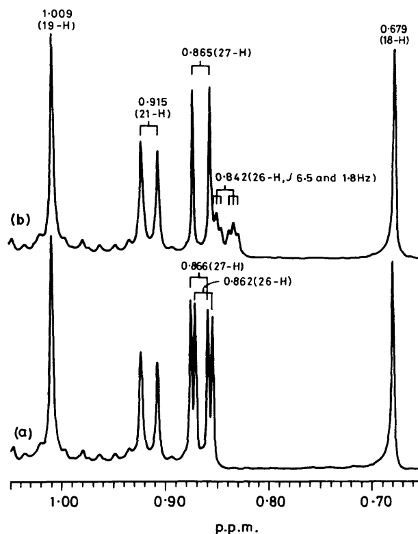
Figure 3. Portion of 400 MHz ^1\text{H} n.m.r. spectra of (a) cholesterol and (b) (25 R )-[26- ^2\text{H} ]cholesterol ( 10 ) recorded on a Varian XL-400 instrument at 23 °C in \text{CDCl}_3
