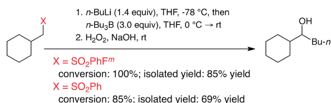
Scheme 2. Example for the Transformation of a m -Fluorophenylsulfone to a Secondary Alcohol a
