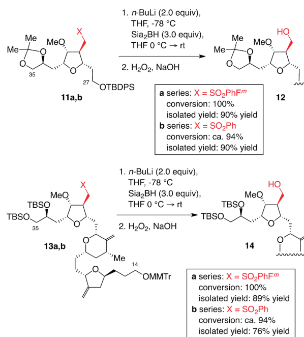
Scheme 3. Application to the C27–C35 and C14–C35 Building Blocks of E7389 a
