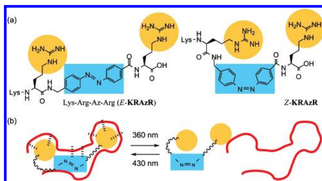
Figure 1. (a) Structures of the E - and Z -isomers of Lys–Arg–Az–Arg ( KRAzR ). Available special orientations for the two guanidinium groups (shown as the orange circles) were dependent on the configuration of azobenzene (shown in the blue rectangles). (b) Illustrations of photoregulation of KRAzR binding to its RNA aptamer (shown as a red line). The dashed lines signify hydrogen bonds to the guanidinium groups and hydrophobic interactions to the azobenzene chromophore.
