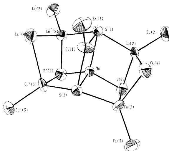
Fig. 1. Perspective view of the [(\text{CuCl})_5\text{Cl}_2\text{MoS}_4]^{4-} anion showing the atom labelling scheme. Half of the anion (primed atoms) is generated through a binary axis passing through \text{Cu}(1) and \text{Cl}(1) .
