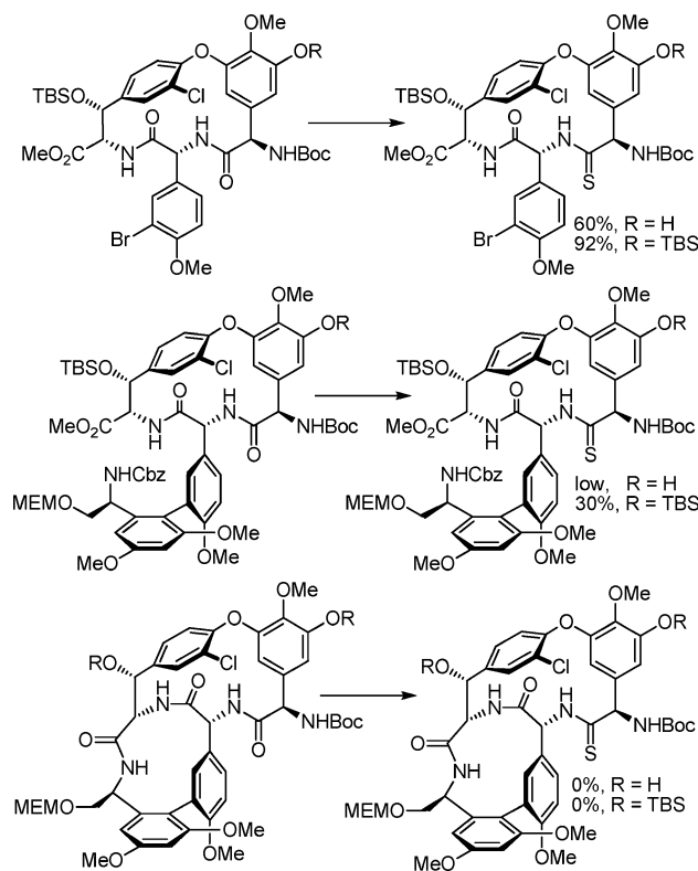
Figure 4. Thionation survey using Lawesson's reagent in toluene.
