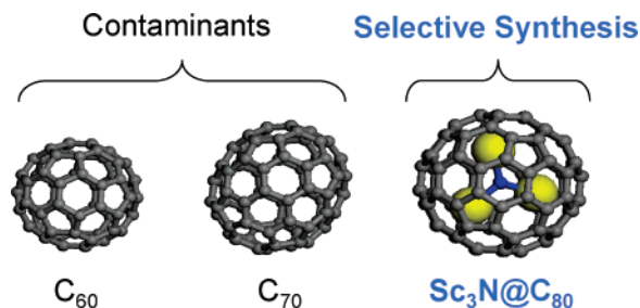
Figure 1. Structures of empty-cage and metallic nitride fullerenes produced in electric-arc soot.
