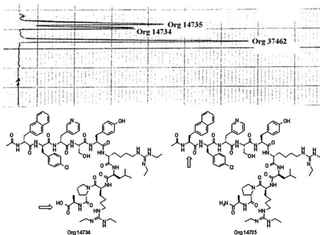
Figure 2. HPLC chromatogram Org 37462, Org 14734 and Org 14735 (HPLC: Symmetry C 18 (5 \mu m 250 \times 4.6 mm) with a gradient of water/acetonitrile/trifluoroacetic acid (90/10/0.1–10/90/0.1, V/V/V), 1 ml/min, 220 nm).
