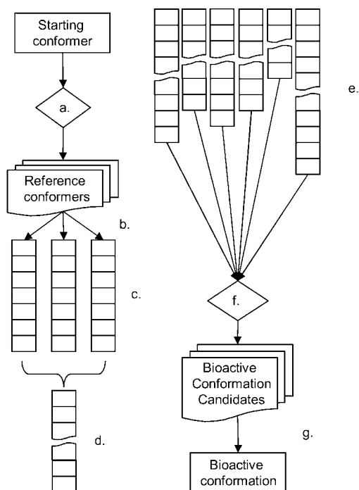
Scheme 1. Generation of the Conformational Ensemble for Each Peptide (a–d) and Selection of the Binding Conformation (e–g) a
