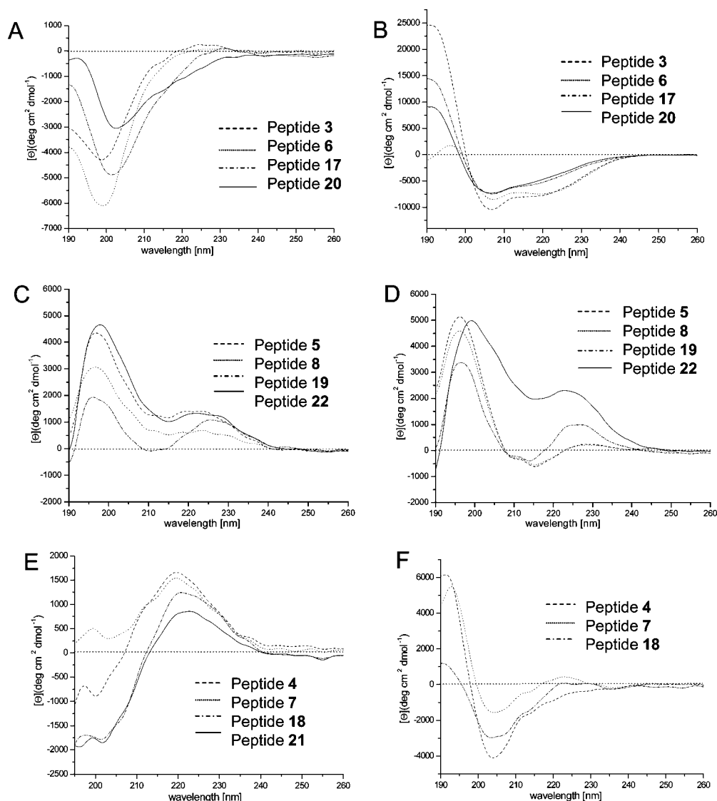
Figure 4. CD spectra of linear and cyclic \beta -amyloid(4–10)-containing epitope peptides in water and in TFE. Linear peptides flanked by \alpha -L-Ala dimers (3) or trimers (6) and their cyclic analogues (17 and 20): (A) in water, (B) in TFE. Linear peptides flanked by \alpha -D-Ala dimers (5) or trimers (8) and their cyclic analogues (19 and 22): (C) in water, (D) in TFE. Linear peptides flanked by \beta -Ala dimers (4) or trimers (7) and their cyclic analogues (18 and 21): (E) in water, (F) in TFE.
