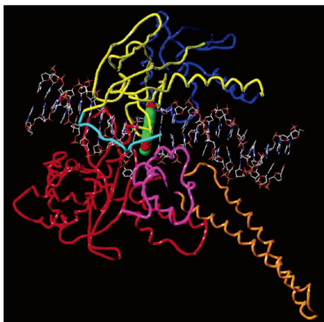
Figure 2. Top: Electron density ( |F_o| - |F_c| at 3.1 Å, contoured at 2\sigma ) showing the initial unbiased experimental density used for the placement of compound 14 into the topo70-DNA covalent complex crystal structure. Bottom: Diagram of the topo70-DNA complex bound with indenoisoquinoline 14 . The topoisomerase I inhibitor 14 is displayed as a space-filling model (CPK). The N-terminal fragment is colored in cyan, the core subdomain I yellow, subdomain II blue, subdomain III red, the linker is orange and the C-terminus is magenta. The oligonucleotide is represented as capped sticks and is colored according to atom type.
