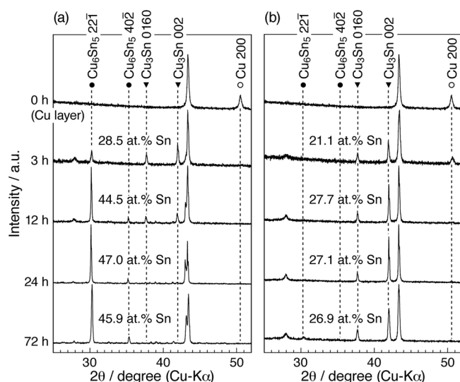
Figure 8. X-ray diffraction patterns and gross compositions of Cu thin layers before and after alloying for 3–72 h at 150°C using \text{EMI-Tf}_2\text{N} bath containing 0.05 \text{ mol dm}^{-3} \text{ Sn(Tf}_2\text{N)}_2 . Alloying potentials were (a) +5 mV and (b) +20 mV vs. Sn rod. Indices of diffraction lines are based on JCPDS No. 45-1488 ( \text{Cu}_6\text{Sn}_5 ), 01-1488 ( \text{Cu}_3\text{Sn} ), and 04-0836 (Cu).
