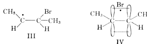
Fig. 2.—Free radical obtained from a mixture of trans -2-butene and HBr. Photolysis about 7 min. at 77°K.
