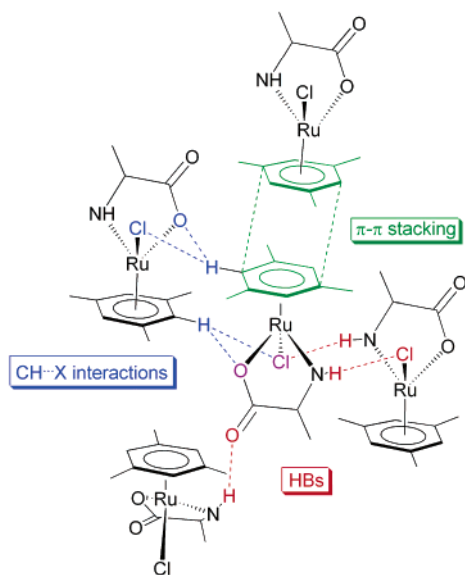
Figure 2. Noncovalent interactions present in the X-ray single-crystal structure of \text{RuCl}(\text{S-Ala})(\text{Mes}) reported by Carter et al. 20
