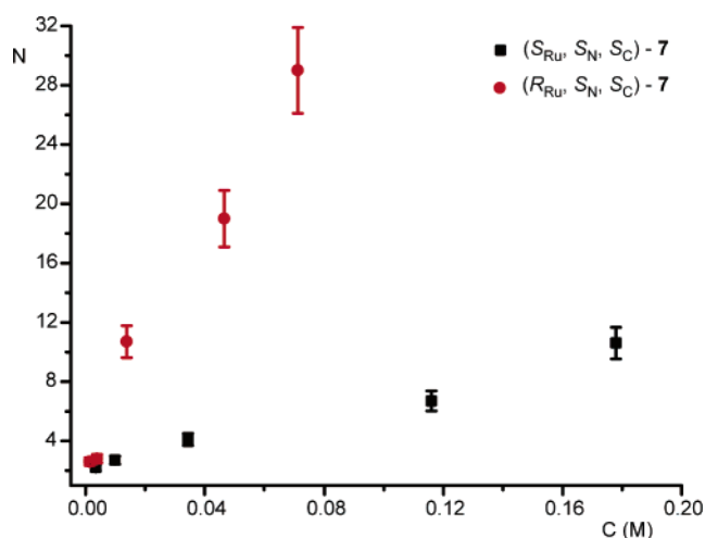
Figure 3. Dependence of the aggregation number ( N ) on the concentration ( C ) for the two diastereoisomers of 7 in \text{CDCl}_3 .
