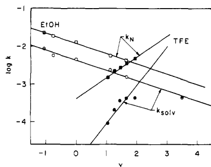
Figure 5. First-order rate constants for solvolysis, k_{\text{solv}} (circles), and second-order rate constants for the reaction with n -propylamine, k_N (squares) of 1c in ethanol–water (50–90%, open symbols), methanol (□, ●), water (●), and trifluoroethanol–water (60–90%, closed symbols), as a function of Y . 23
