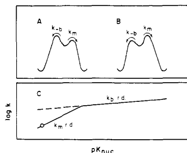
Figure 9. Reaction coordinate diagram for (A) rate-limiting bond breaking ( k_m > k_b ) and (B) rate-limiting bond making ( k_b > k_m ) in the mechanism of eq 3. As the nucleophile becomes weaker, there will be a change in the rate-limiting step from k_b to k_m (C).
