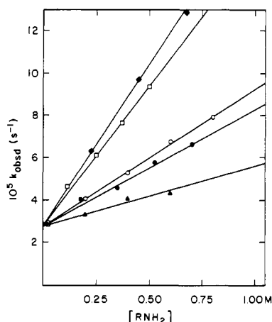
Figure 2. Pseudo-first-order rate constants for the reactions of N -(methoxymethyl)- N,N -dimethyl- m -bromanilinium ion ( 1b ) with primary amines at 25 °C, ionic strength 1.0 M (KCl): n -propylamine, ■; methoxyethylamine, □; hydroxylamine, ○; 1,1-dimethylethylenediamine, ●; methoxyamine, ▲.
