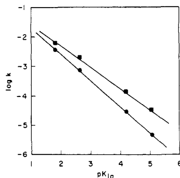
Figure 8. Dependence on the pK_a of the leaving dimethylaniline of the rate constants for reactions of ring-substituted N -(methoxymethyl)- N , N -dimethylanilinium ions with water (●) and with n -propylamine (■).
