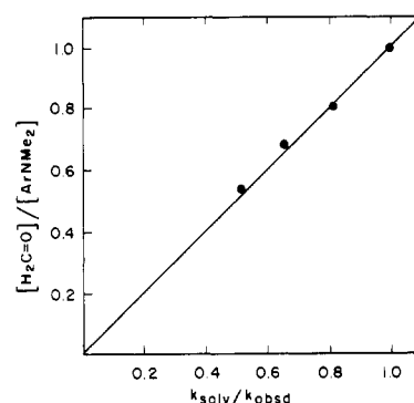
Figure 3. Comparison of product and rate constant ratios for the reaction of N -(methoxymethyl)- N,N -dimethyl- m -nitroanilinium ion ( 1c ) with triethylenediamine at 25 °C and ionic strength 1.0 M (KCl). The ordinate describes the fraction of the total reaction products as formaldehyde, and the abscissa gives the ratio of the rate constant for hydrolysis to the observed rate constant in the presence of different concentrations of amine.
