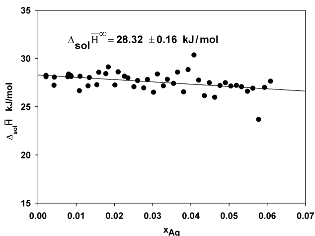
Fig. 1. Molar enthalpies of solution of Ag in a liquid Sn-bath at 773 K. The extrapolated value at infinite dilution ( x_{\text{Ag}} = 0 ) is given.
