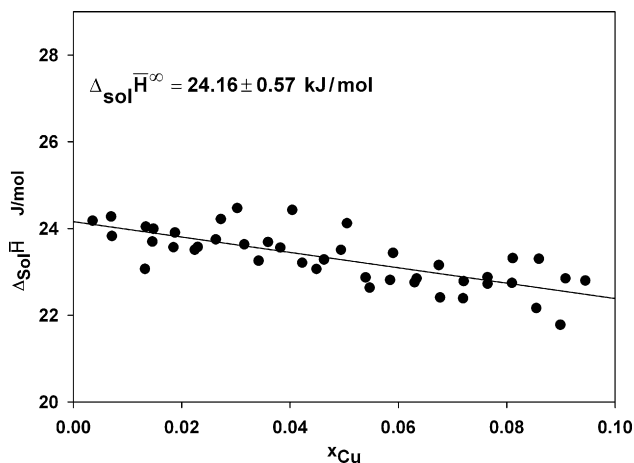
Fig. 2. Molar enthalpies of solution of Cu in a liquid Sn-bath at 773 K. The extrapolated value at infinite dilution ( x_{\text{Cu}} = 0 ) is given.
