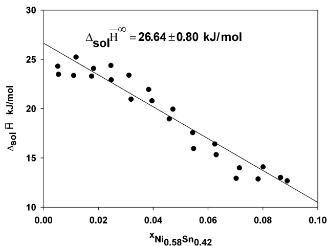
Fig. 6. Molar enthalpies of solution of \text{Ni}_{0.58}\text{Sn}_{0.42} in a liquid Sn-bath at 773 K. The extrapolated value at infinite dilution ( x_{\text{Comp.}} = 0 ) is given.
