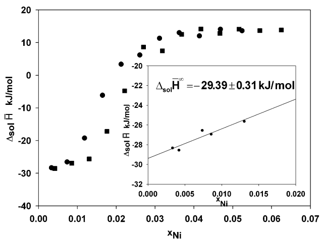
Fig. 3. Molar enthalpies of solution of Ni in a liquid Sn-bath at 773 K. The inset shows the composition range x_{\text{Ni}} \leq 0.02 where the bath is single phase. The extrapolated value at infinite dilution ( x_{\text{Ni}} = 0 ) is given.
