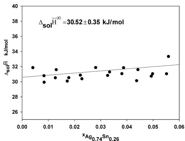
Fig. 4. Molar enthalpies of solution of \text{Ag}_{0.74}\text{Sn}_{0.26} in a liquid Sn-bath at 773 K. The extrapolated value at infinite dilution ( x_{\text{Comp.}} = 0 ) is given.
