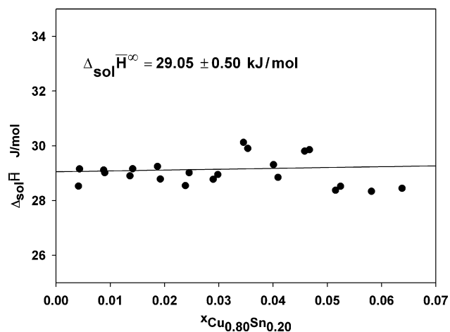
Fig. 5. Molar enthalpies of solution of \text{Cu}_{0.80}\text{Sn}_{0.20} in a liquid Sn-bath at 773 K. The extrapolated value at infinite dilution ( x_{\text{Comp.}} = 0 ) is given.
