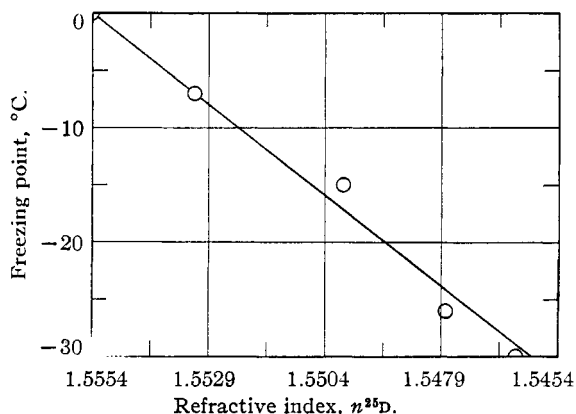
Fig. 2.—Plot of the refractive indices against the freezing points of mixtures of the isomeric monobromocyclooctadienes II and III.
