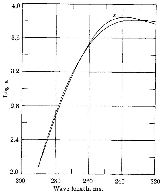
Fig. 5.—Ultraviolet absorption spectra of dibromocyclooctadiene: curve 1, sample prepared from 1,5-cyclooctadiene and N-bromosuccinimide; curve 2, sample prepared from 1,3,5-cyclooctatriene and bromine.
