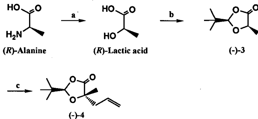
Scheme 4. Reagents and conditions: a. \text{NaNO}_2 , 1 N \text{H}_2\text{SO}_4 ; b. 2,2-dimethylpropanal, p\text{-TsOH} , conc. \text{H}_2\text{SO}_4 in pentane; c. LDA, allyl bromide in THF.
