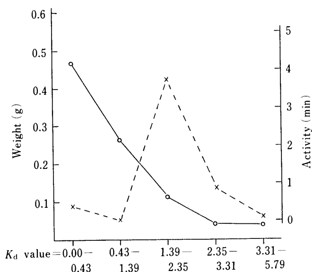
Fig. 1. Elution Pattern of the AcOEt Layer (1.436 g) on Sephadex LH-20 Gel Filtration (4.1 x 45 cm Column)
