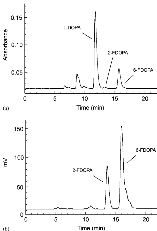
Figure 2 Typical analytical HPLC UV (a) and radiochromatogram (b) for a reaction mixture resulting from the direct fluorination of L-DOPA in 99% \text{CF}_3\text{SO}_3\text{H} at -40^\circ\text{C} .
