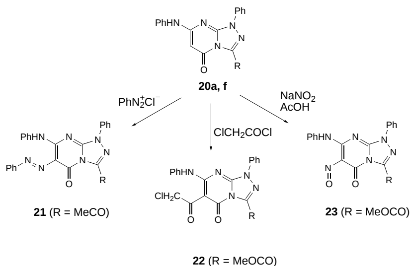
Scheme 5
