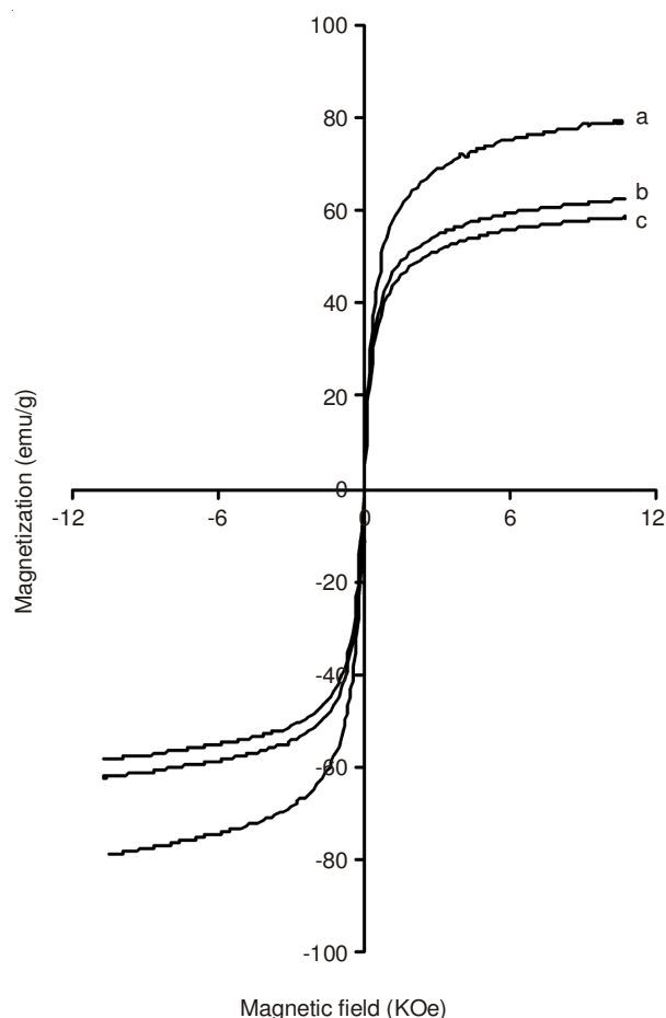
Fig. 5. Magnetization curves of MNPs (a) and PMMA coated particles synthesized with different MMA/magnetite ratios: (b) 8/1, (c) 16/1
