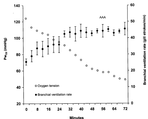
Fig. 1. Relationship between water oxygen tension ( PwO_2 ), branchial ventilation rate (gill strokes per minute) and the onset of air breathing. Each letter 'A' signifies a single air breath. Vertical bars are mean values \pm 1 S.D.
