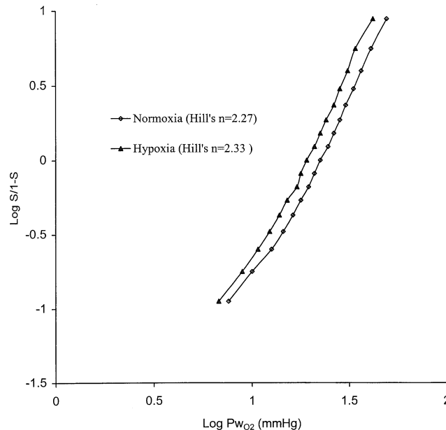
Fig. 3. Hill plots for oxygen equilibrium curves of blood from eight lungfish N. forsteri exposed to normoxic and moderately hypoxic conditions for at least 14 days ( P_{CO_2} = 16 mmHg, T_w = 20^\circ\text{C} ). O_2 equilibrium data are mean values plotted from 0.05 to 0.95 saturation at 0.05 increments. Mean pH values were 7.7 \pm 0.3 in hypoxic conditions and 7.5 \pm 0.3 in normoxic conditions.
