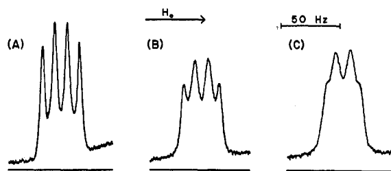
Figure 1.—The \text{SiH}_2 resonance in the ^1\text{H} nmr spectrum of 1\text{-(ClSiH}_2\text{)}_2\text{B}_5\text{H}_8 at 34^\circ (A), -71^\circ (B), and -85^\circ (C).
