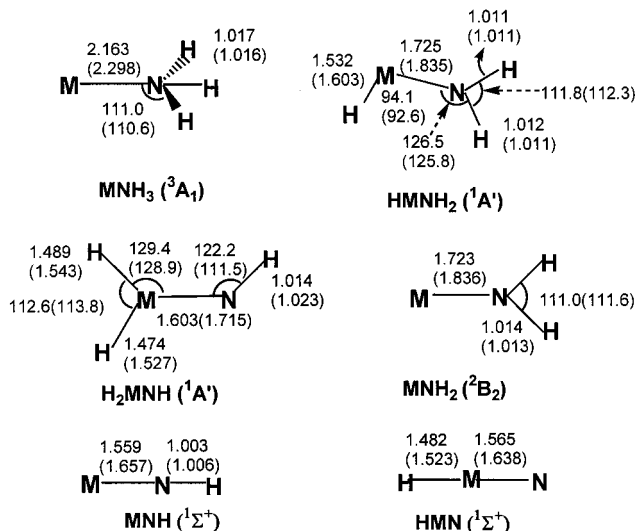
Figure 5. Calculated geometric parameters (bond lengths in angstroms, bond angles in degrees) of the \text{MNH}_3 , \text{HMNH}_2 , \text{H}_2\text{MNH} , \text{MNH} , and \text{NMH} ( \text{M} = \text{Si} and \text{Ge} ) molecules. Values for \text{Ge} compounds are listed in parentheses.
