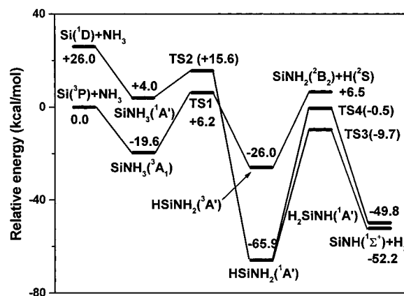
Figure 6. Potential energy surface along the Si + \text{NH}_3 reaction path calculated at the B3LYP/6-311++G(d,p) level. Energies are given in kcal/mol and are relative to the reactants \text{Si}(^3\text{P}) + \text{NH}_3(^1\text{A}_1) .
