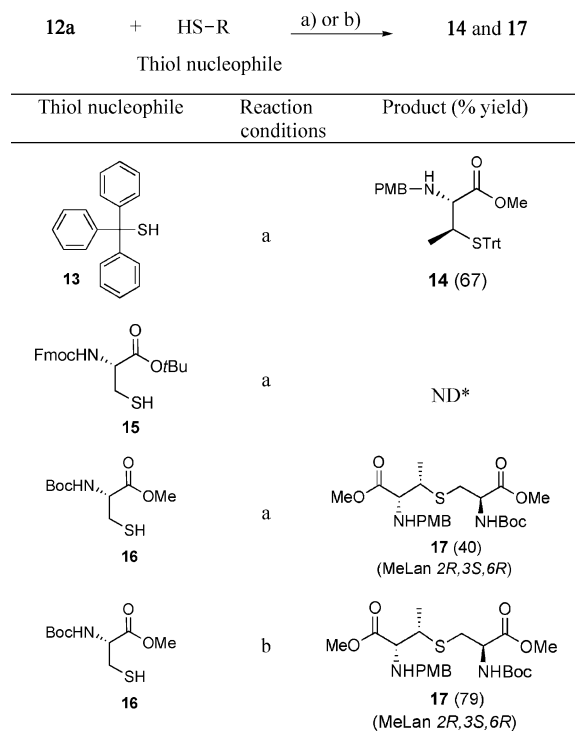
Fig. 3 Initial sulfamidate ring opening reactions. Reagents and conditions: a) (i) \text{Cs}_2\text{CO}_3 , DMF, rt, (ii) 1 M \text{NaH}_2\text{PO}_4 buffer pH 5.4, rt; b) (i) \text{Cs}_2\text{CO}_3 , DMF, rt, (ii) n\text{PrSH}/\text{BF}_3 \cdot \text{Et}_2\text{O} , \text{CH}_2\text{Cl}_2 , rt, then \text{NH}_4\text{OH} , rt. * No formation of the desired product was detected.
