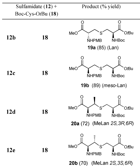
Fig. 4 Preparation of orthogonally protected Lan 19a and 19b and \beta -MeLan 20a and 20b . Reagents and conditions: a) (i) \text{Cs}_2\text{CO}_3 , DMF, rt, (ii) n\text{PrSH}/\text{BF}_3 \cdot \text{Et}_2\text{O} , \text{CH}_2\text{Cl}_2 , rt, then \text{NH}_4\text{OH} , rt.
