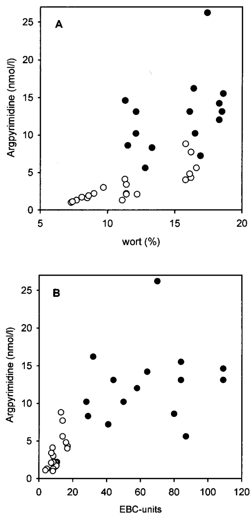
Figure 4. Correlation of Argpyrimidine concentration in beer to wort content (A) and beer color expressed as EBC units (B). Closed circles indicate samples with EBC units of more than 28.
