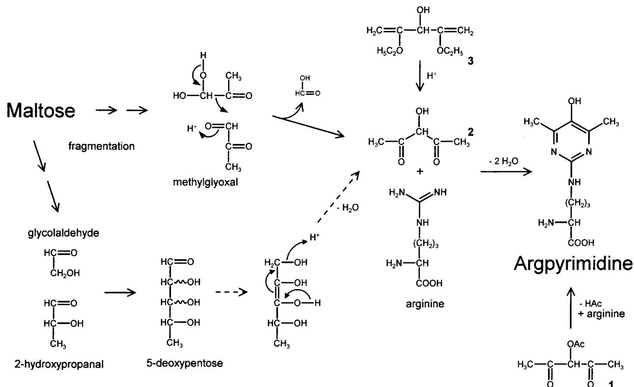
Figure 1. Mechanisms of Argpyrimidine formation from maltose.
