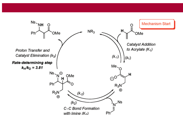
Figure 2. Proposed catalytic cycle for the aza-MBH reaction as reported by Jacobsen. The quoted KIE, with xylenes as the reaction solvent, is for the acrylate α-proton (bold).
