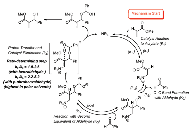
Figure 1. Proposed catalytic cycle for the MBH reaction in the absence of protic additives as reported by McQuade and Aggarwal. Quoted KIEs are for the acrylate α-proton (bold).
