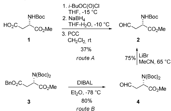
SCHEME 3. Synthesis \beta -Keto Ester 5
