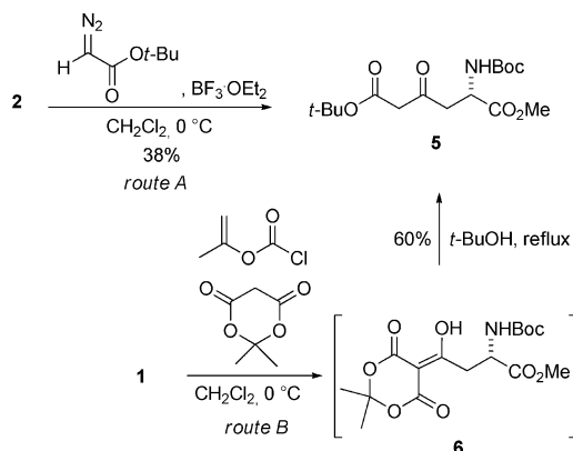
SCHEME 3. Synthesis \beta -Keto Ester 5
