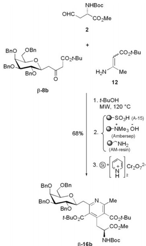
SCHEME 6. Synthesis of 2-(C-Galactosylmethyl)-4-(alaninyl)pyridine \beta -16b
