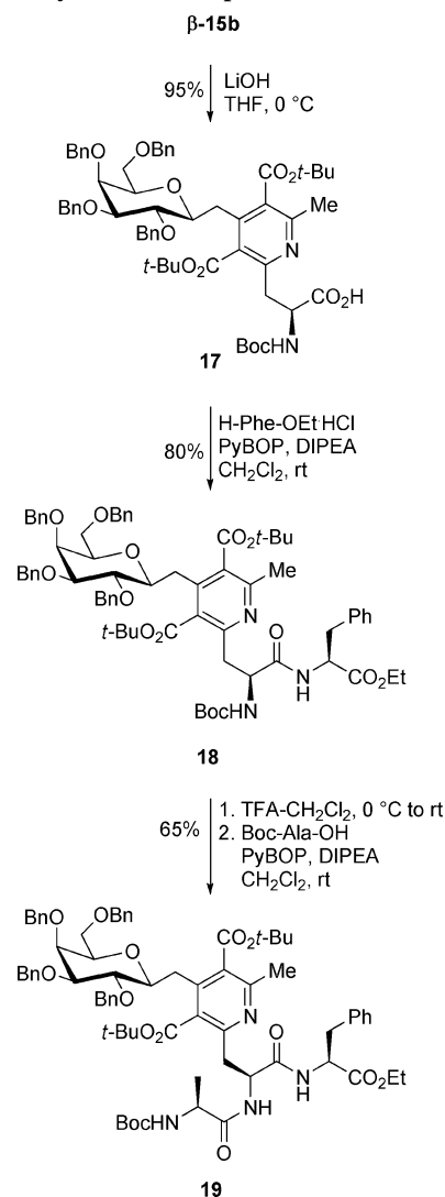
SCHEME 7. Synthesis of Tripeptide 19
