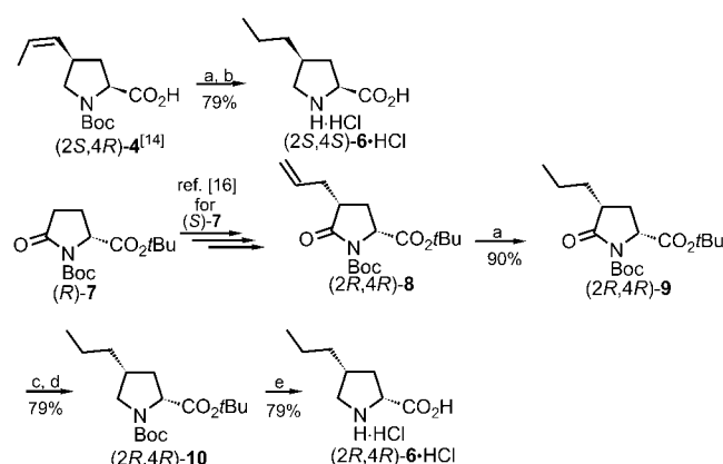
Scheme 2. Synthesis of both enantiomers of cis -4-propylproline ( 6 ). a) H 2 , Pd/C, EtOAc, 20 °C, 15 h; b) 2 M HCl/EtOAc, 20 °C, 1 h; c) LiEt 3 H, THF, −78 °C, 1 h; d) Et 3 SiH, BF 3 ·Et 2 O, CH 2 Cl 2 , −78 °C, 2.5 h; e) 6 M HCl, 85 °C, 2 h.
