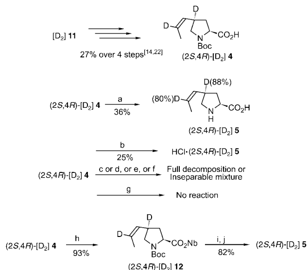
Scheme 4. The final stages in the preparation of the doubly deuterium-labeled amino acid (2 S ,4 R )-[D] 5 . a) TFA (neat), 20°C, 20 min, then 15 lyophilisations from water; b) 5 N HCl/Et 2 O, 20°C, 4 h; c) BF 3 ·Et 2 O, CH 2 Cl 2 , 20°C, 1 h; d) TMSI, CH 2 Cl 2 , 0°C, 30 min; e) TFA/Me 2 S/CH 2 Cl 2 , 0°C, 1 h; f) SnCl 4 , CH 2 Cl 2 , 20°C, 2 h; g) 180°C, 30 min; h) p -O 2 N-PhCH 2 Br, K 2 CO 3 , MeCN, 70°C, 3 h; i) 5 N HCl/Et 2 O, 20°C, 3 h; j) 1 N NaOH, 0°C, 30 min, then 1 N HCl.
