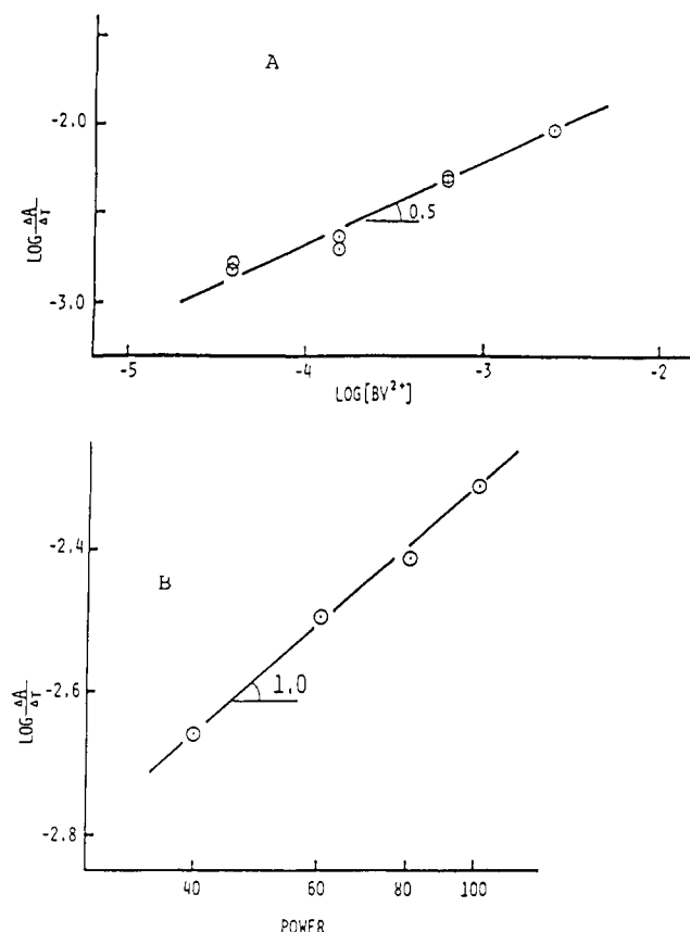
Figure 3. Logarithmic dependences of the rate of reduction on BV^{2+} concentration (A) and plasma power (B).
