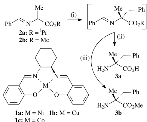
Scheme 1. Reagents: (i) 1a–c (2–10 mol%)/NaOH (solid)/BnBr; (ii) \text{H}_3\text{O}^+/\Delta ; (iii) (R=Me), MeOH/AcCl then \text{SiO}_2 .
