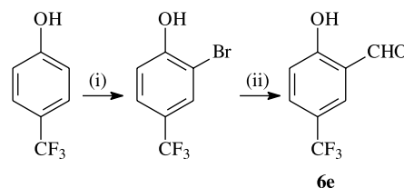
Scheme 3. Reagents: (i) \text{Br}_2 ; (ii) \text{BuLi}/\text{DMF} .
