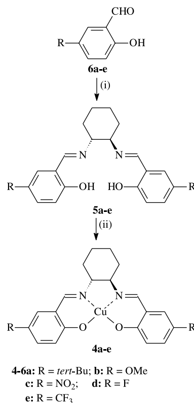
Scheme 2. Reagents: (i) ( R,R )-cyclohexane diamine/NaOMe; (ii) \text{CuBr}_2/\text{NaOMe} .
